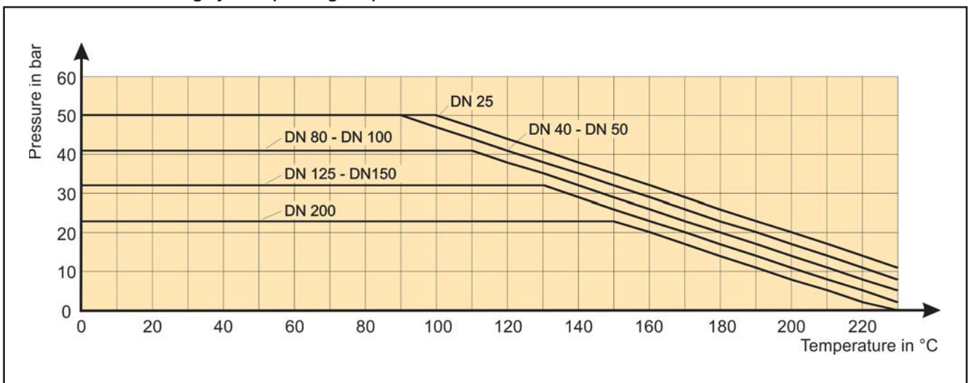
Fig. 10 - Pressure-temperature diagram
