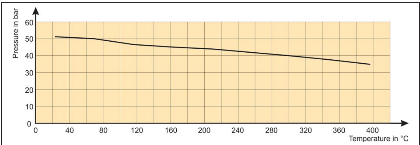
Fig. 13 - Pressure-temperature diagram
