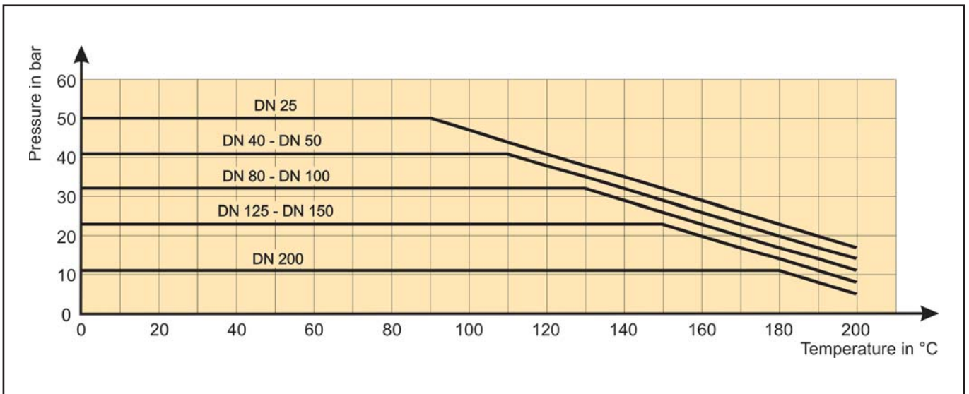
Fig. 9 - Pressure-temperature diagram
