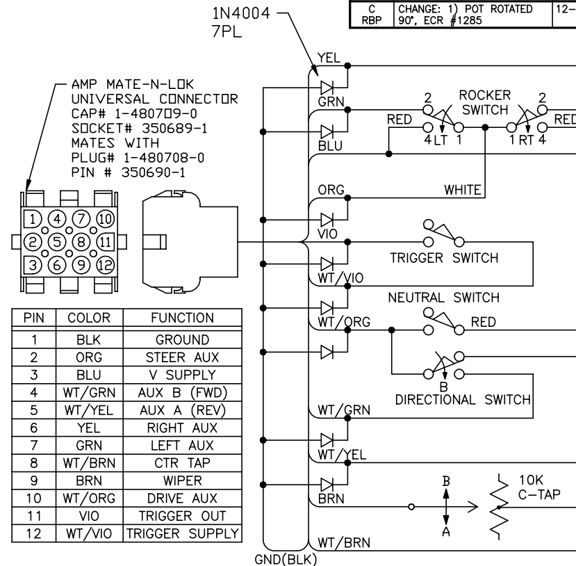
ELECTRICAL CONNECTION
