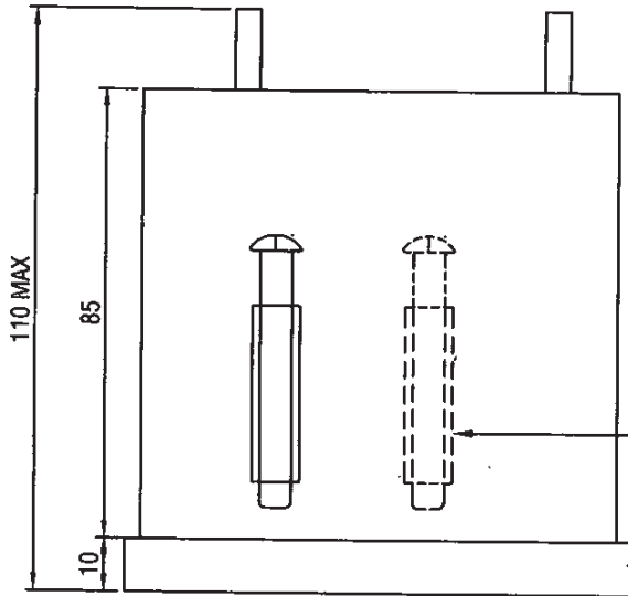
DETACHABLE MOUNTING CLAMP WITH SCREW - 2nos
